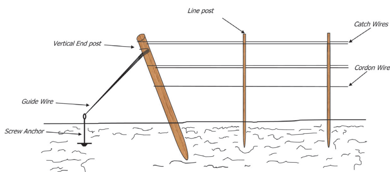
Figure 1. Anchored end post assembly. (All drawings not to scale.)
