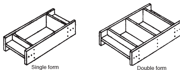
Figure 1. Common forms for molding adobe brick.
