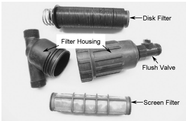
Figure 4. Example of types of filters used in small plot, drip-irrigation systems.
